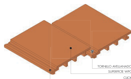
DETALLE 3D - Arkowood wallpanel exterior
